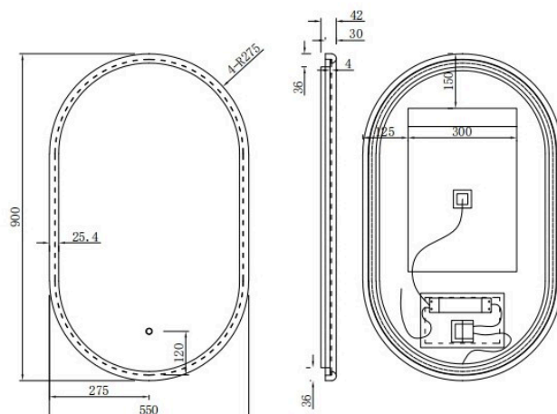
JA25016-LED Mirror
